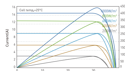
I-V/P-V Curve at different Irradiation (440W)
