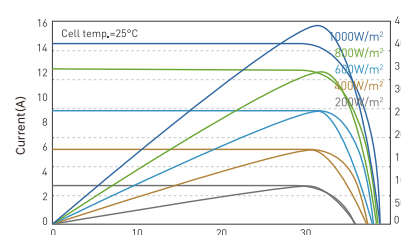
I-V/P-V Curve at different Irradiation (440W)
